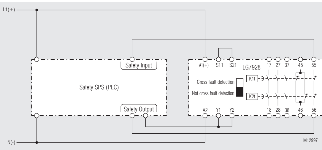
Safety PLC with LG 7928, non cross fault detection, suitable up to SIL 2, Performance Level d, Cat. 3
