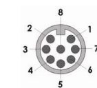
Quick Connect Pin View from Switch
