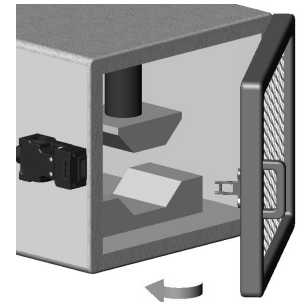
Hinged Guard
