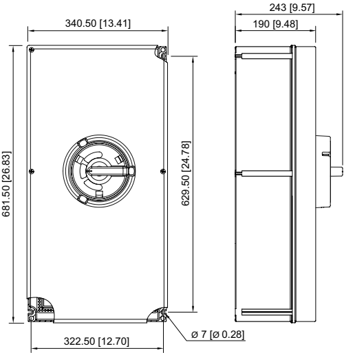
Switching arrangement 8544/1-4 and 8549/1-4
