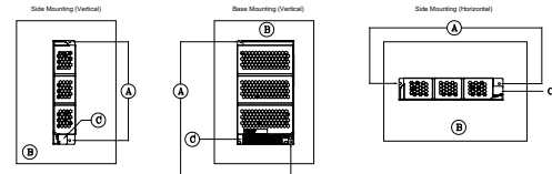
Figure 2 - Mounting
