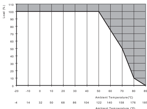
Power Derating Curve for PSU
