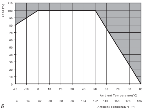
Power Derating Curve for PSU
