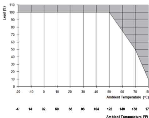
Power Derating Curve for PSU
