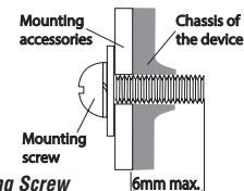
Figure 4 - Mounting Screw
