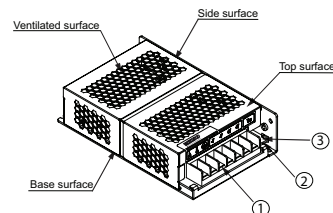
Figure 1 - Device Descriptions
