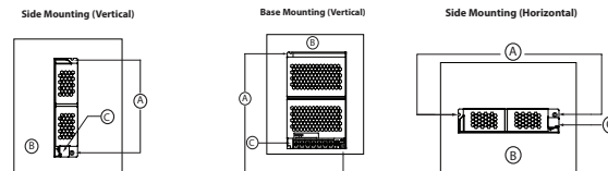
Figure 2 - Mounting
