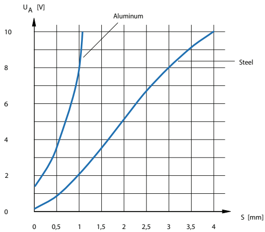
Response diagram
