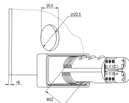
Fig. 2 Mounting cutout
