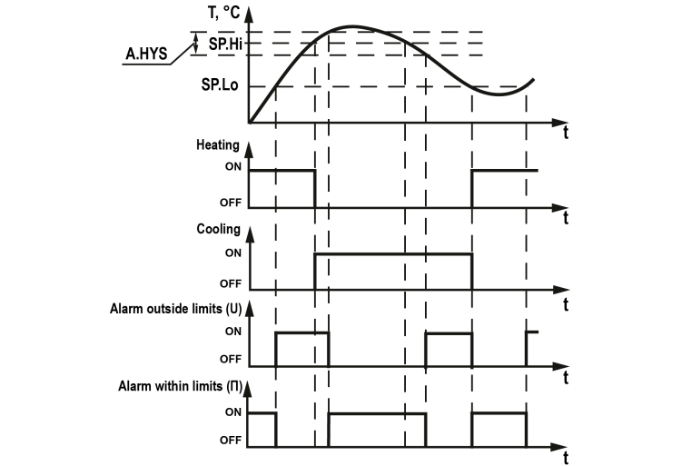
Fig. 10 Output device logic
