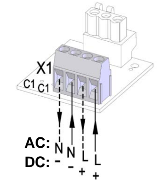
Operating voltage connection
