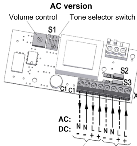
Operating voltage connection for sounder Operating voltage connection for flashing light
