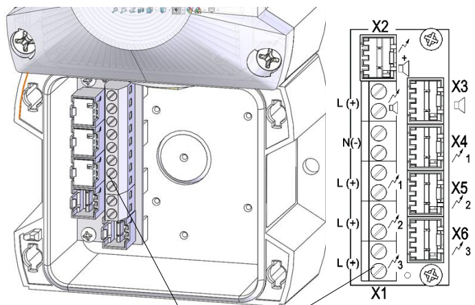
Borne (X1) de raccordement
