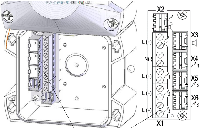
Connecting terminal (X1)
