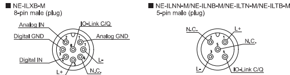
M12 Connector Pin Configuration
