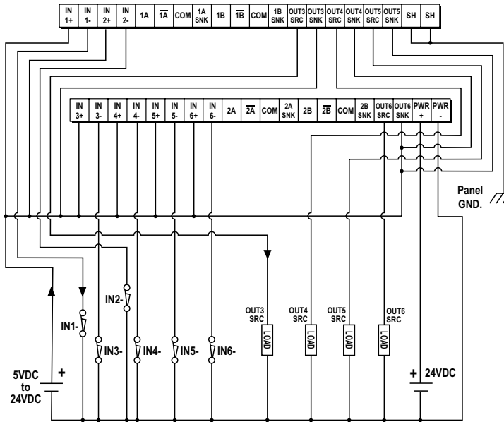
Sourcing I/O Wiring Diagram
