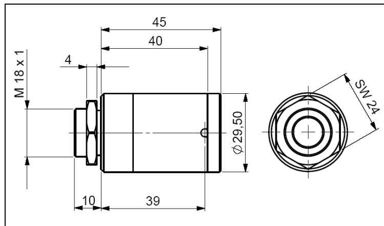
Sensing head [LT15HS]
