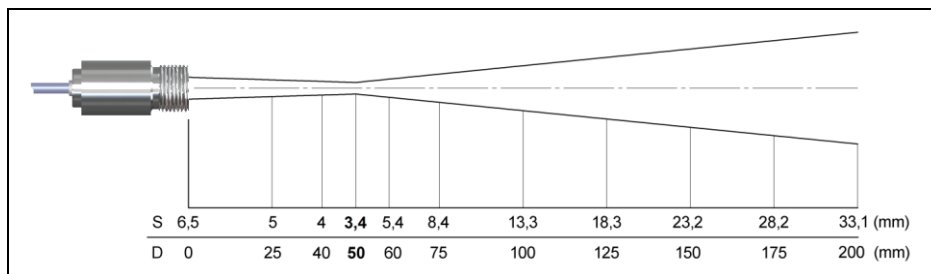
LT15CF/ LT15HCF D:S = 15:1 / D:S \text{ Far field} = 5:1
