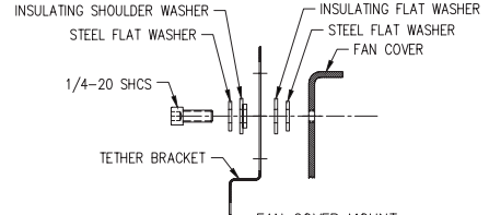
FAN COVER MOUNT WITH THREADED HOLE
