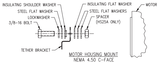
TETHER OPTION "E", "M"
