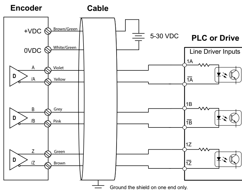
Line Driver Wiring
