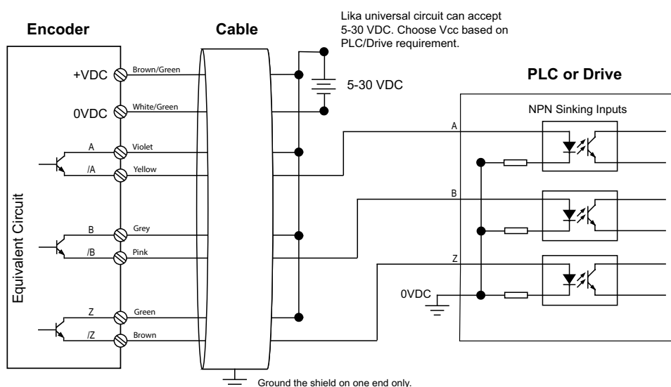
Sinking Input Wiring
