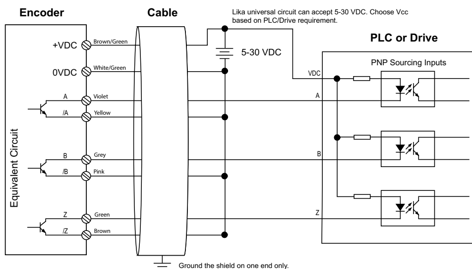
Sourcing Input Wiring
