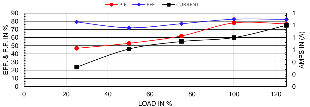
OUTPUT VS EFF., P.F. & CURRENT CURVE
