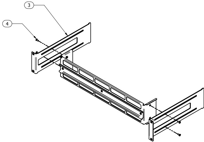
STEP 2 - Rail mounting flange assembly
