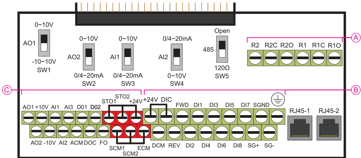
Control circuit board is removable from the GS4 (for ease of wiring)
