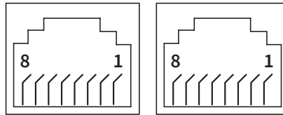
GS4 Serial Comm Ports (2) RS-485 Interface
