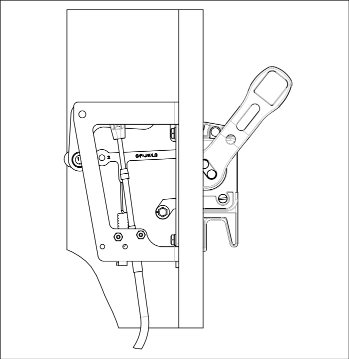
Figure 6. Assembly of Adapter Link to Bell Crank.
