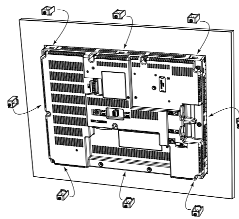
EA9-T12CL, EA9-T15CL and EA9-T15CL-R (8 places)
