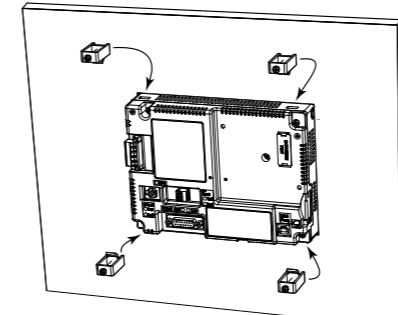
EA9-T6CL, EA9-T6CL-R, EA9-T7CL, EA9-T7CL-R, EA9-T8CL and EA9-T10WCL (4 places)
