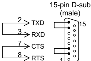
Wiring Diagram
