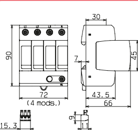
Dimension drawing
