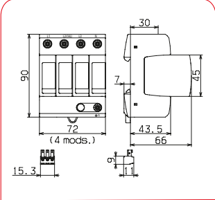
Dimension drawing
