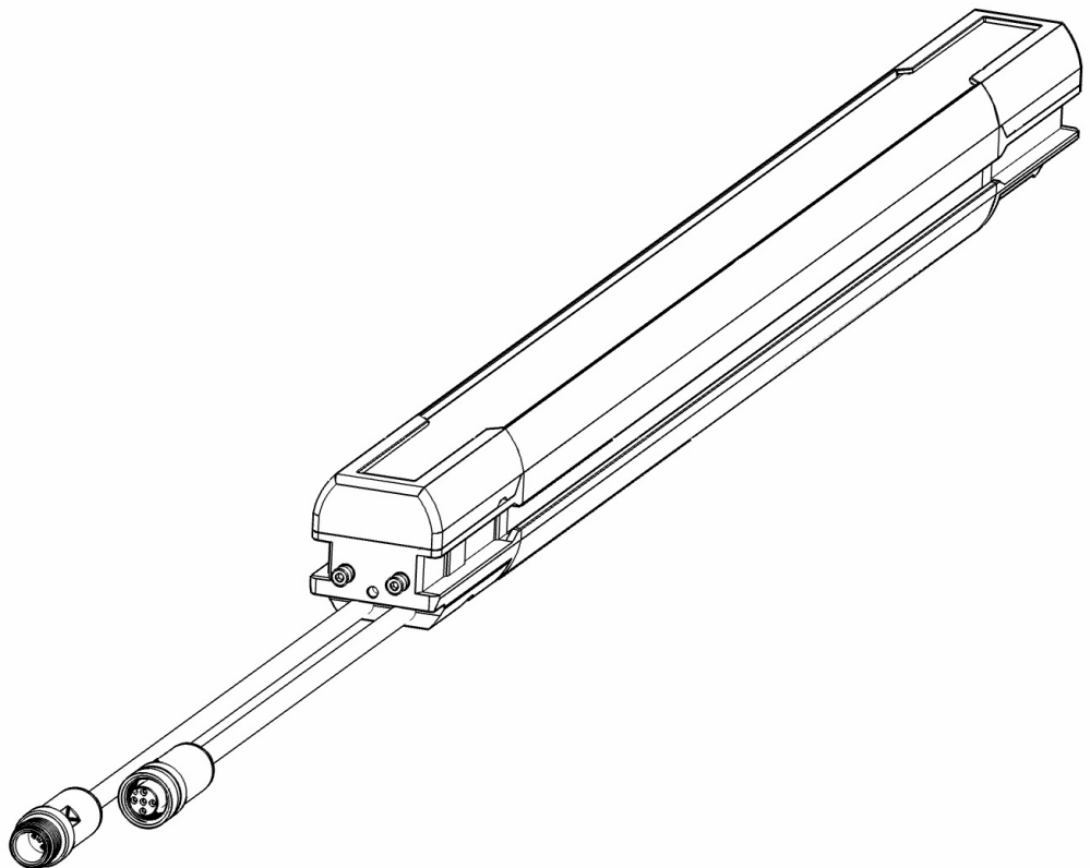
Figure 1: Connections
