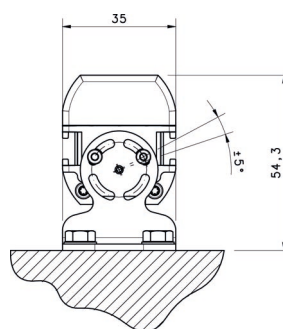
Figure 14 - Straight mounting
