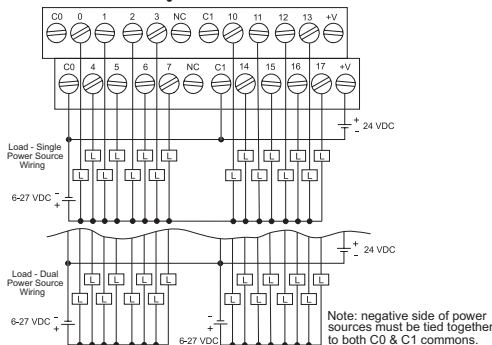
Wiring for D0-16TD1
