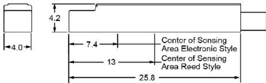
ELECTRONIC SWITCH DIMENSIONS
