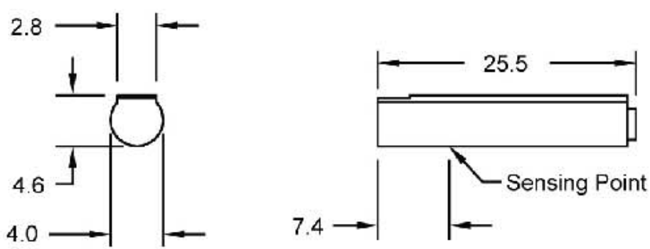
ELECTRONIC SWITCH DIMENSIONS
