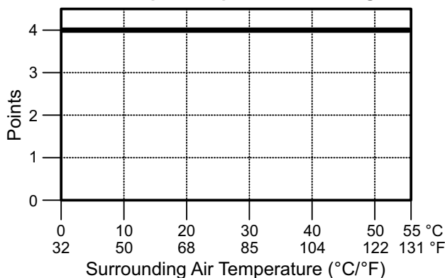
Discrete Output Temperature Derating Chart
