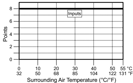
C0-00AR-D Temperature Derating Chart
