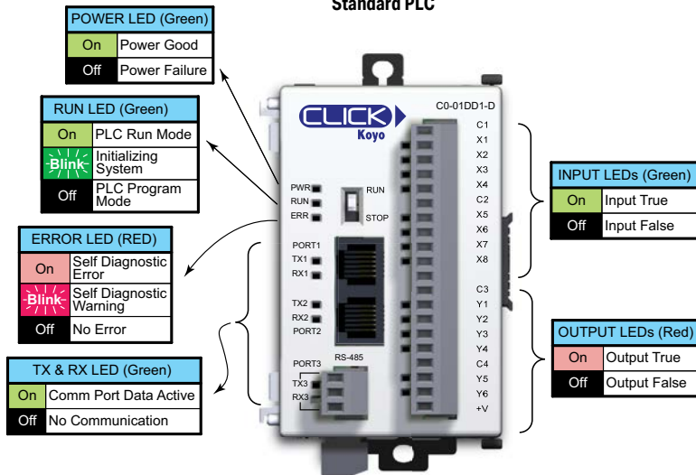
Standard PLC
