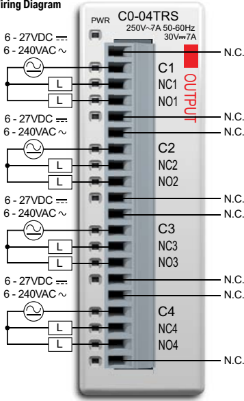
Wiring Diagram
