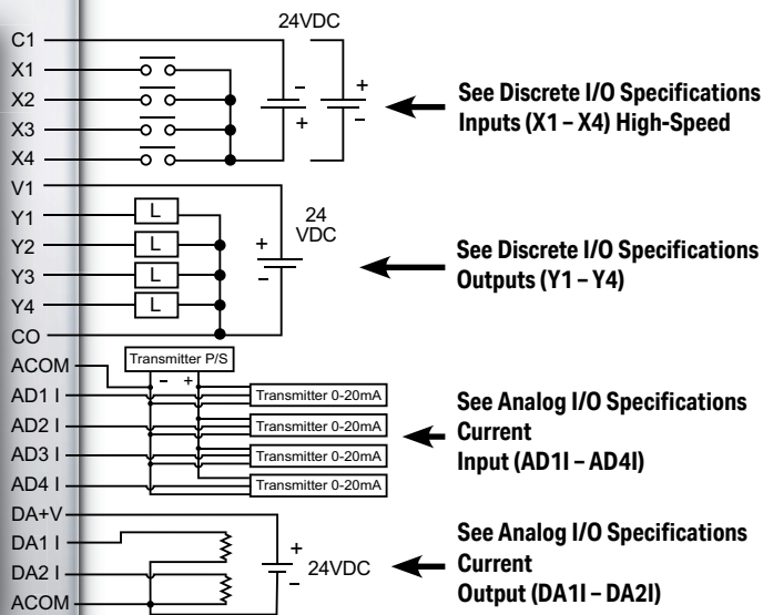
Wiring Diagram
