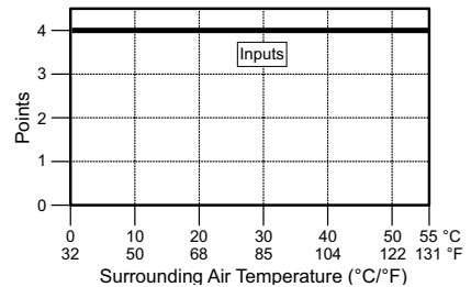
C0-12DD2E-1-D Temperature Derating Chart
