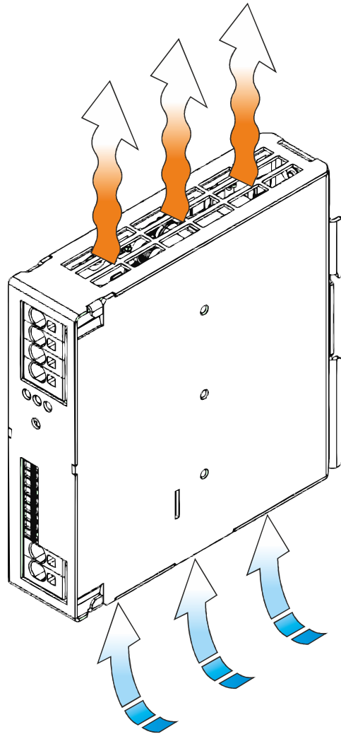
Figure 8: Convection cooling
