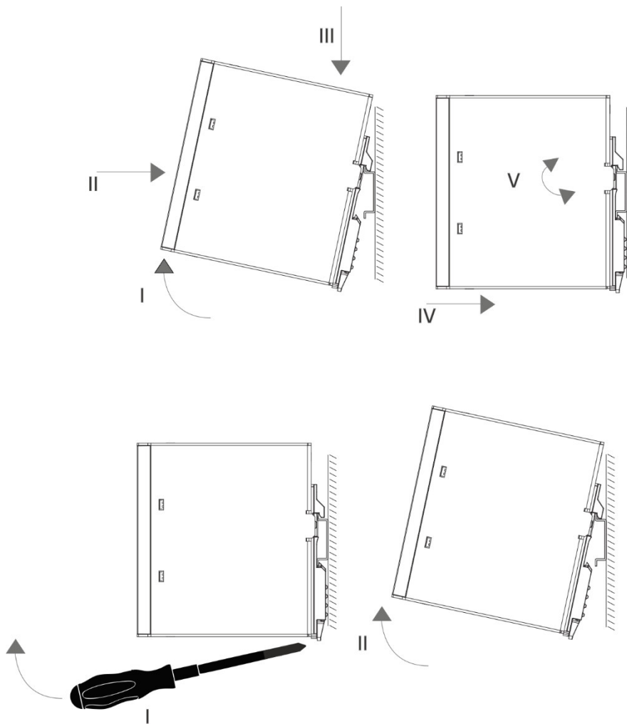
Figure 7: Assembly
