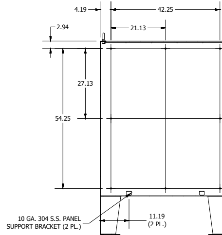
SECTION A-A (INSIDE BACK OF ENCL.)
