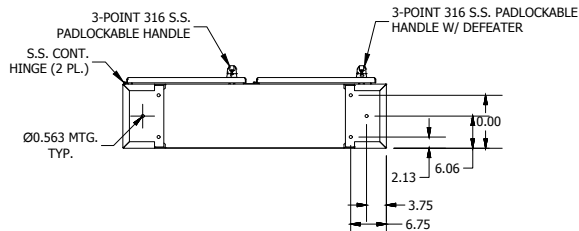
BOTTOM VIEW
