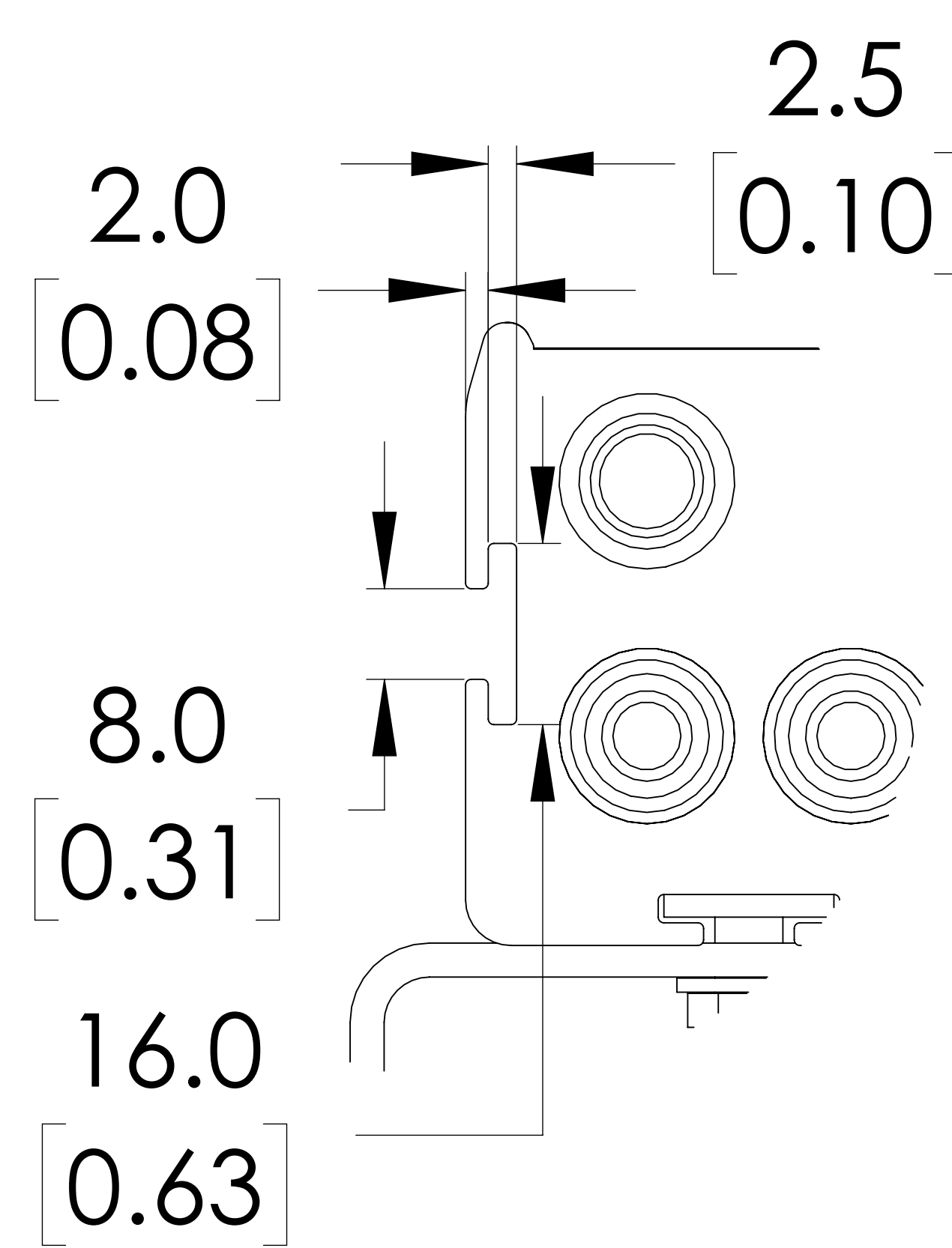
DETAIL A SCALE 2 : 1
