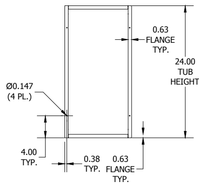
FRONT VIEW LID REMOVED
