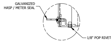
DETAIL A (METER SEAL DETAIL)
