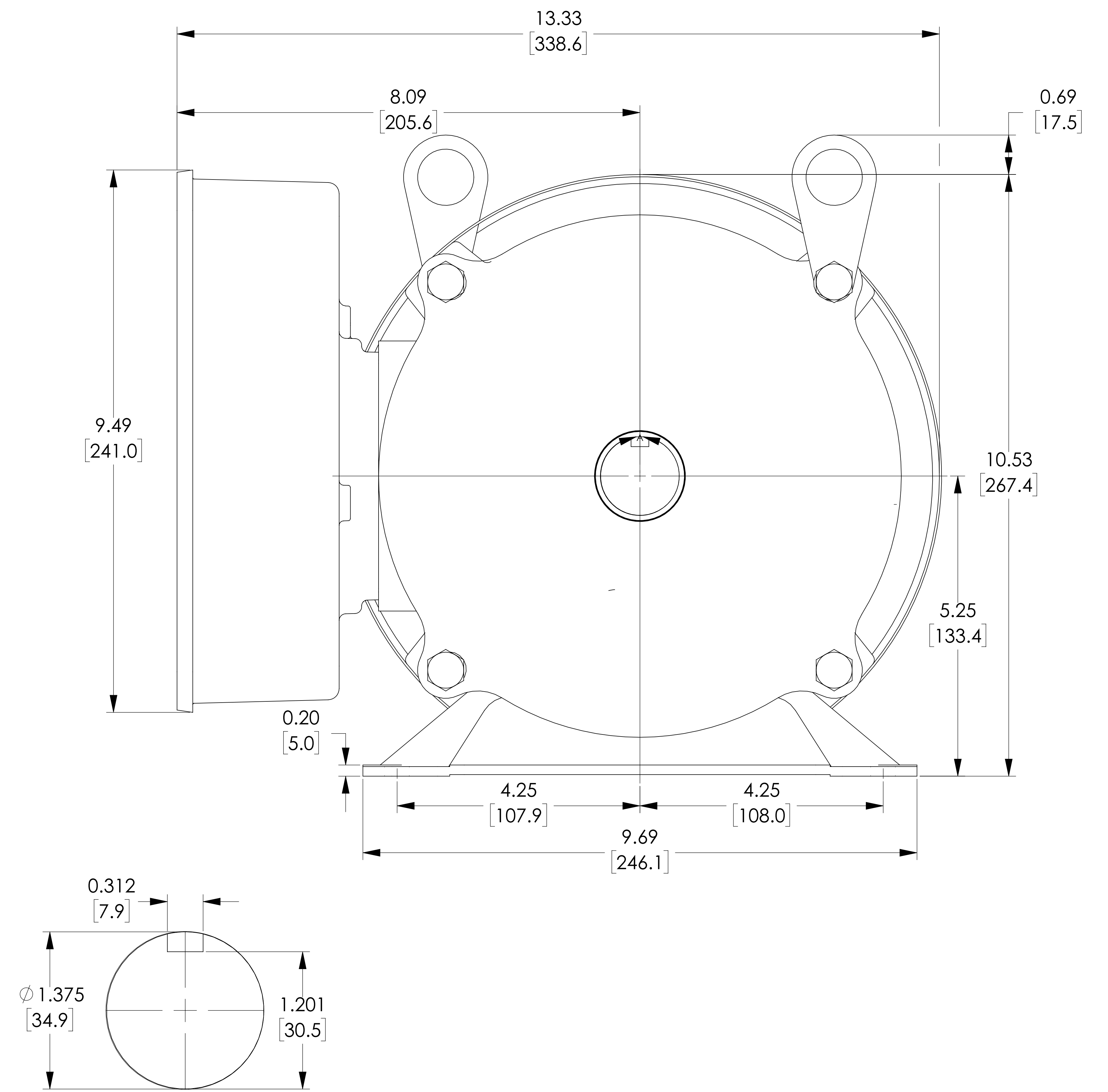
DETAIL A SCALE 2 : 1
