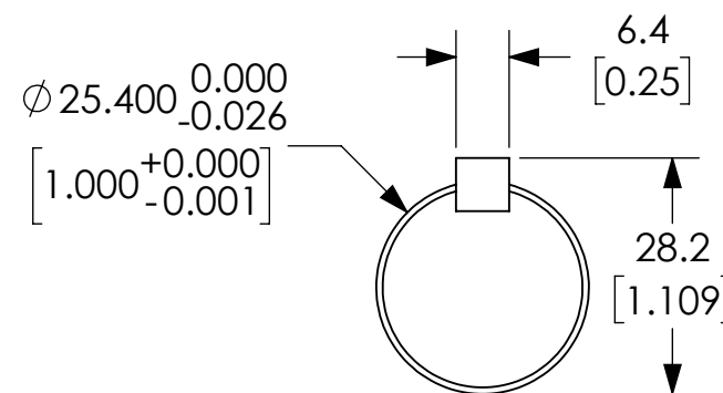
OUTPUT SHAFT SCALE 2:1
