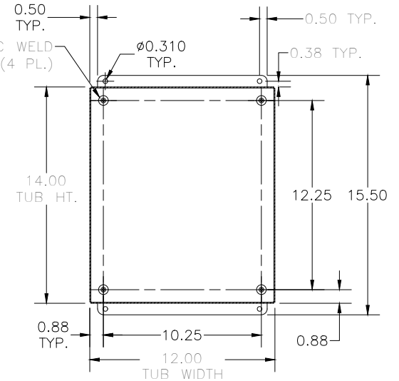
SECTION F-F (INSIDE BACK VIEW)
