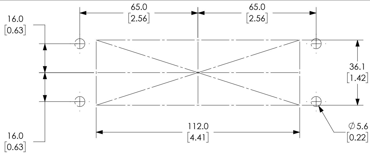
PANEL CUTOUT DETAIL
