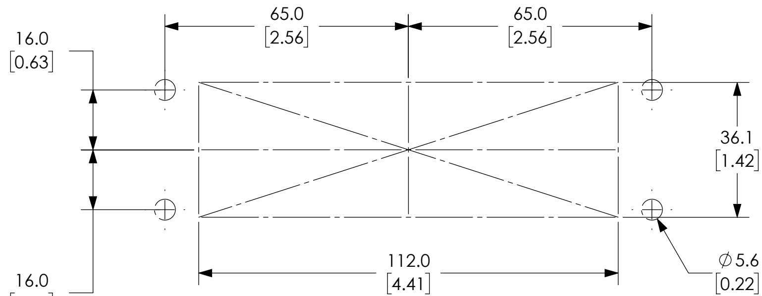
PANEL CUTOUT DETAIL
