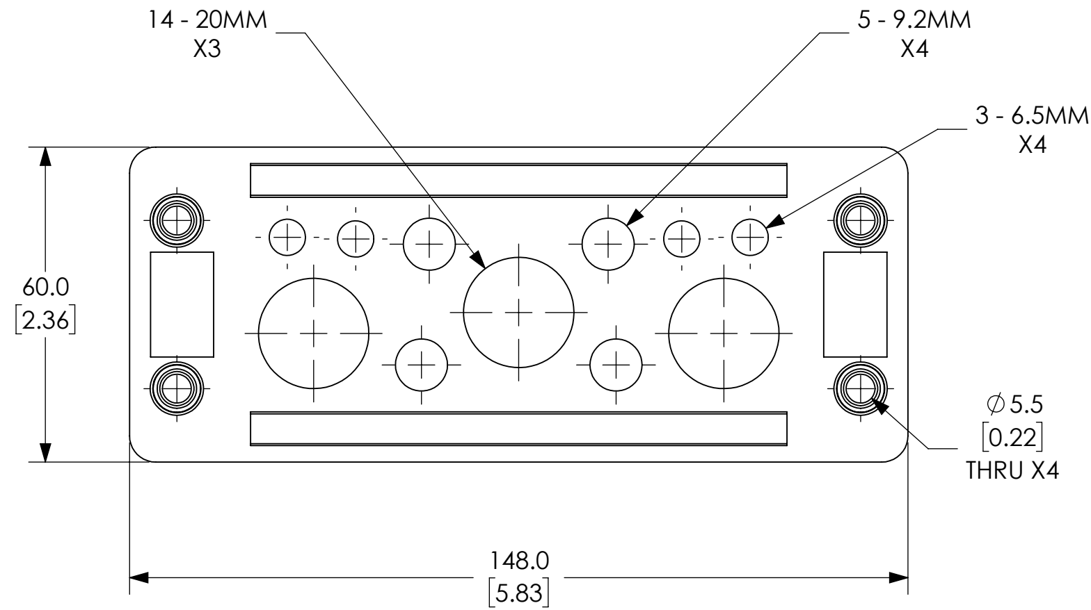
PANEL CUTOUT DETAIL
