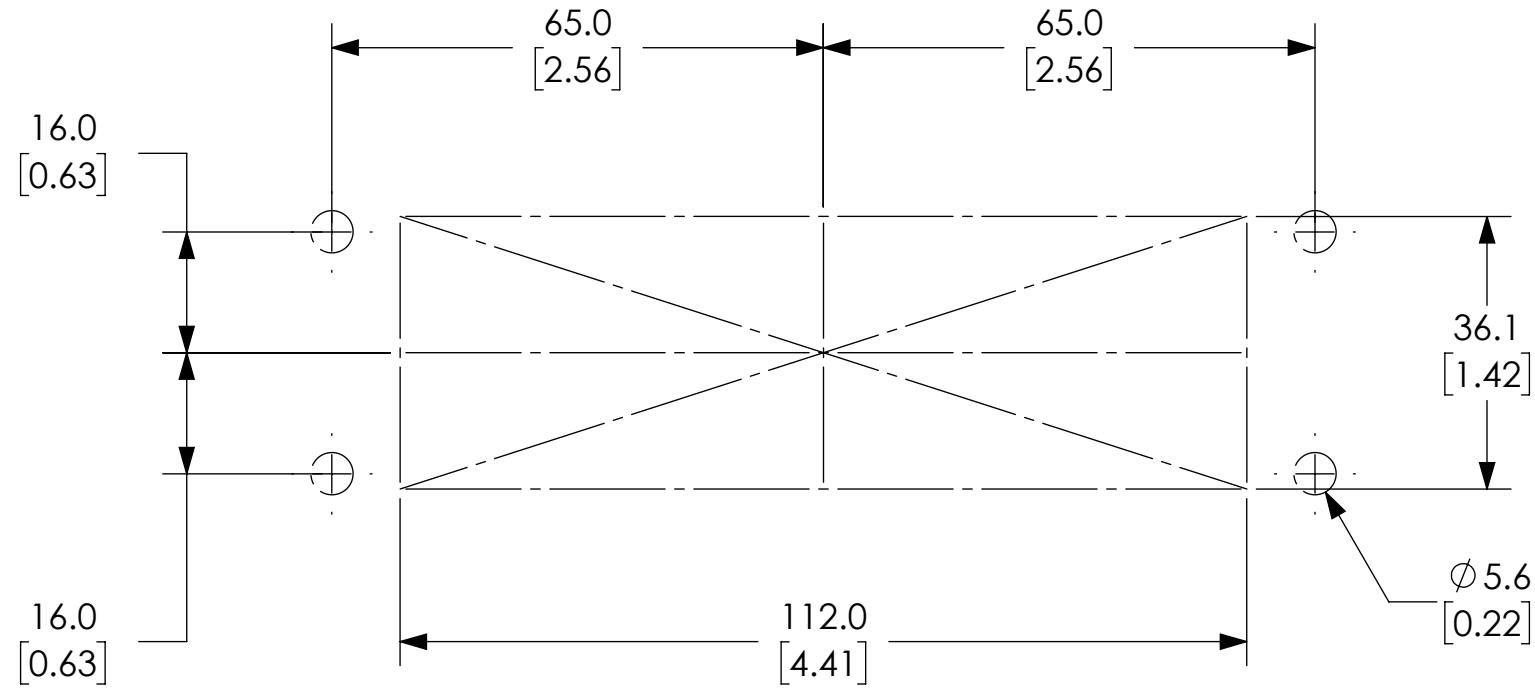
PANEL CUTOUT DETAIL
