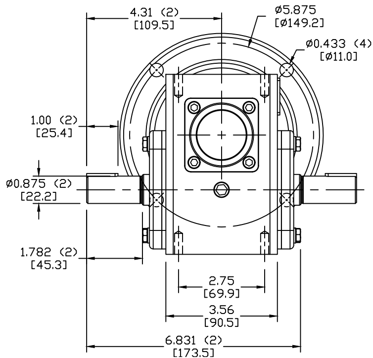
REAR VIEW
