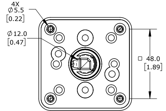
SECTION A-A MOUNT TEMPLATE DIMENSIONS
