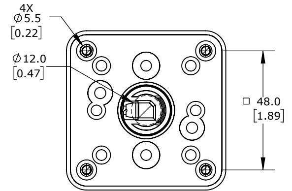
SECTION A-A MOUNT TEMPLATE DIMENSIONS
