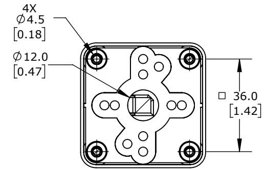
SECTION A-A MOUNT TEMPLATE DIMENSIONS
