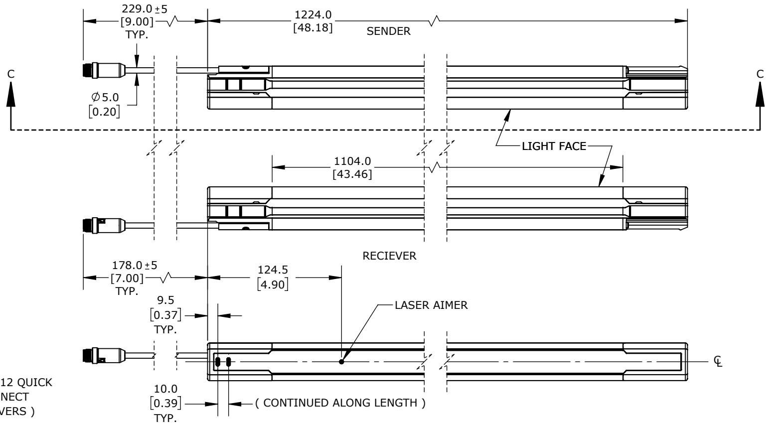
SECTION C-C
