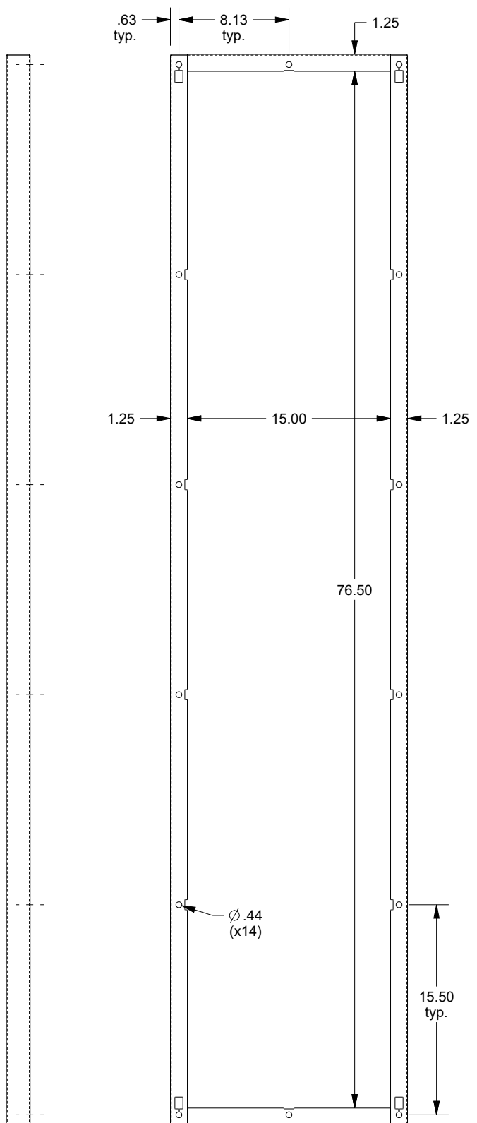
REAR VIEW
