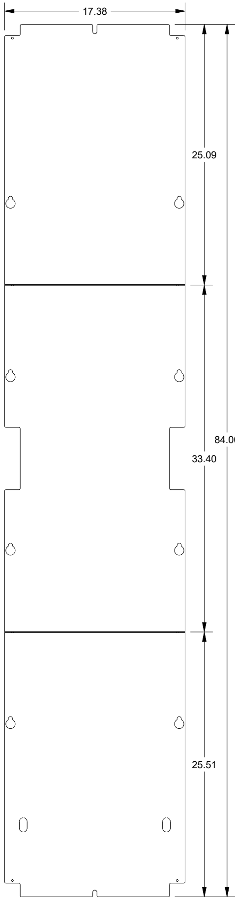
FRONT VIEW
