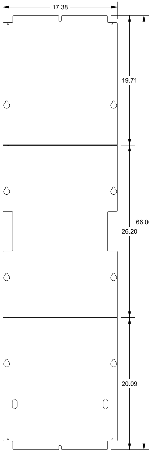
FRONT VIEW
